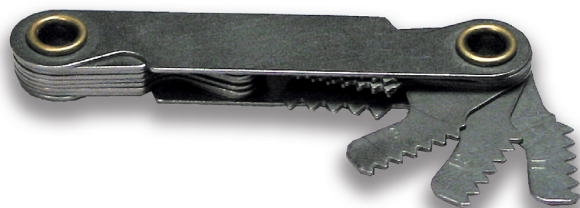
TYPE 730 SCREW PITCH GAUGES
